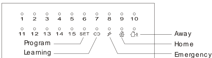
LED display for wireless zones
